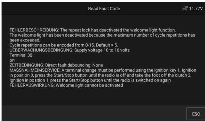
Figure 4-19 Sample Read Fault Codes Screen 3
