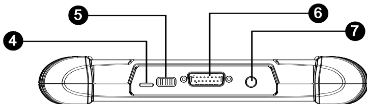
Figure 2-3 CR MAX Display Tablet Top View
