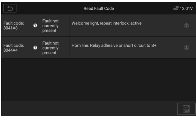
Figure 4-17 Sample Read Fault Codes Screen 1
