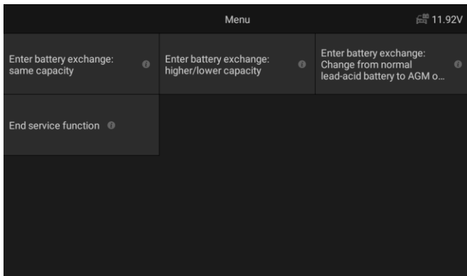
Figure 5-38 Sample BMS Function Screen 6
